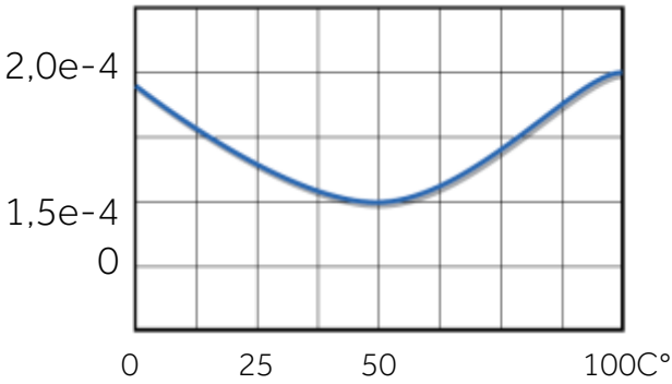
Tang. Delta
