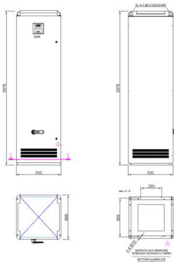
Cabinet for floor mounting
