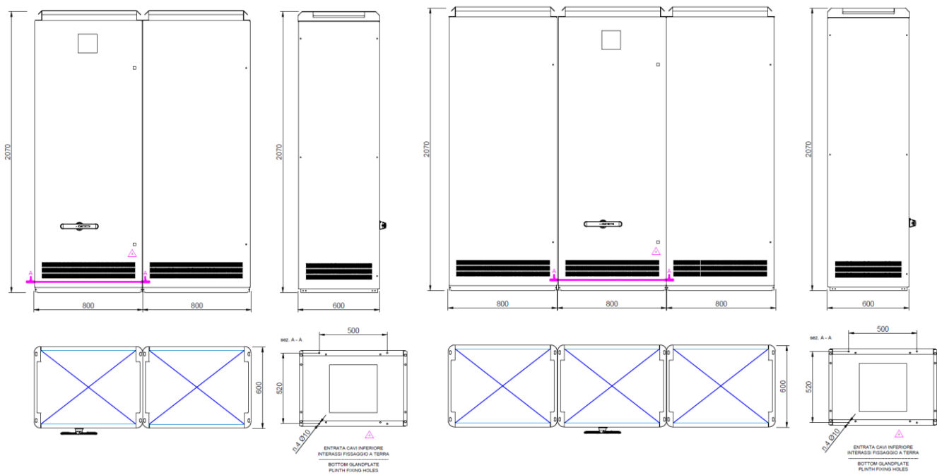
2-door cabinet:
