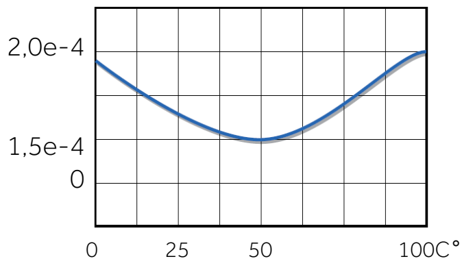
Tang. Delta
