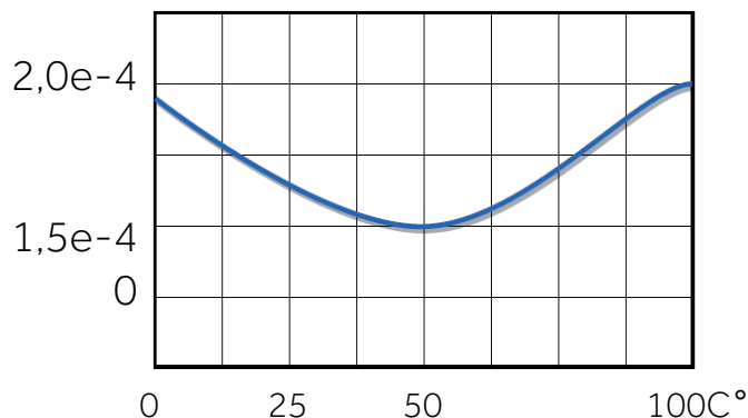
Tang. Delta
